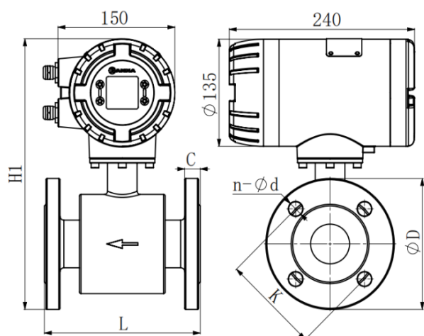
Integrated transmitter
