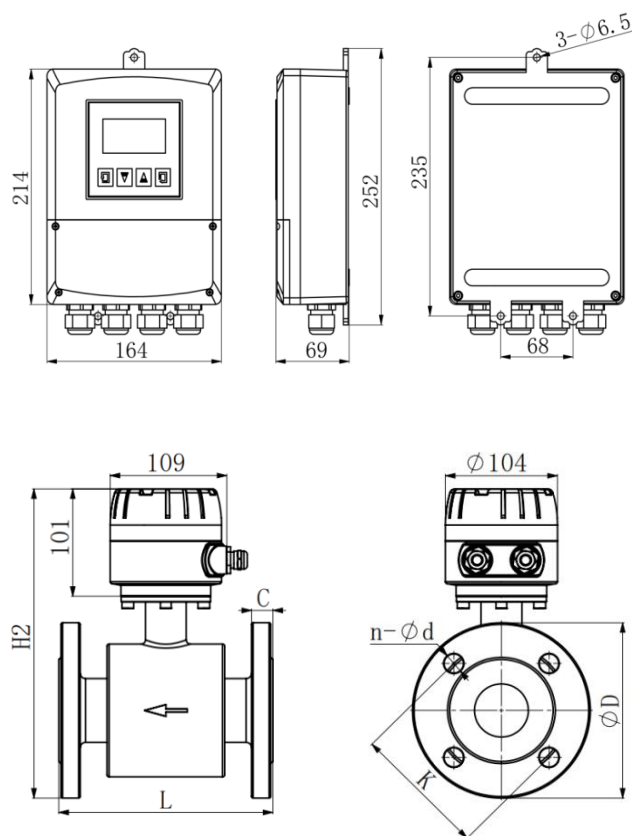
Remote transmitter
